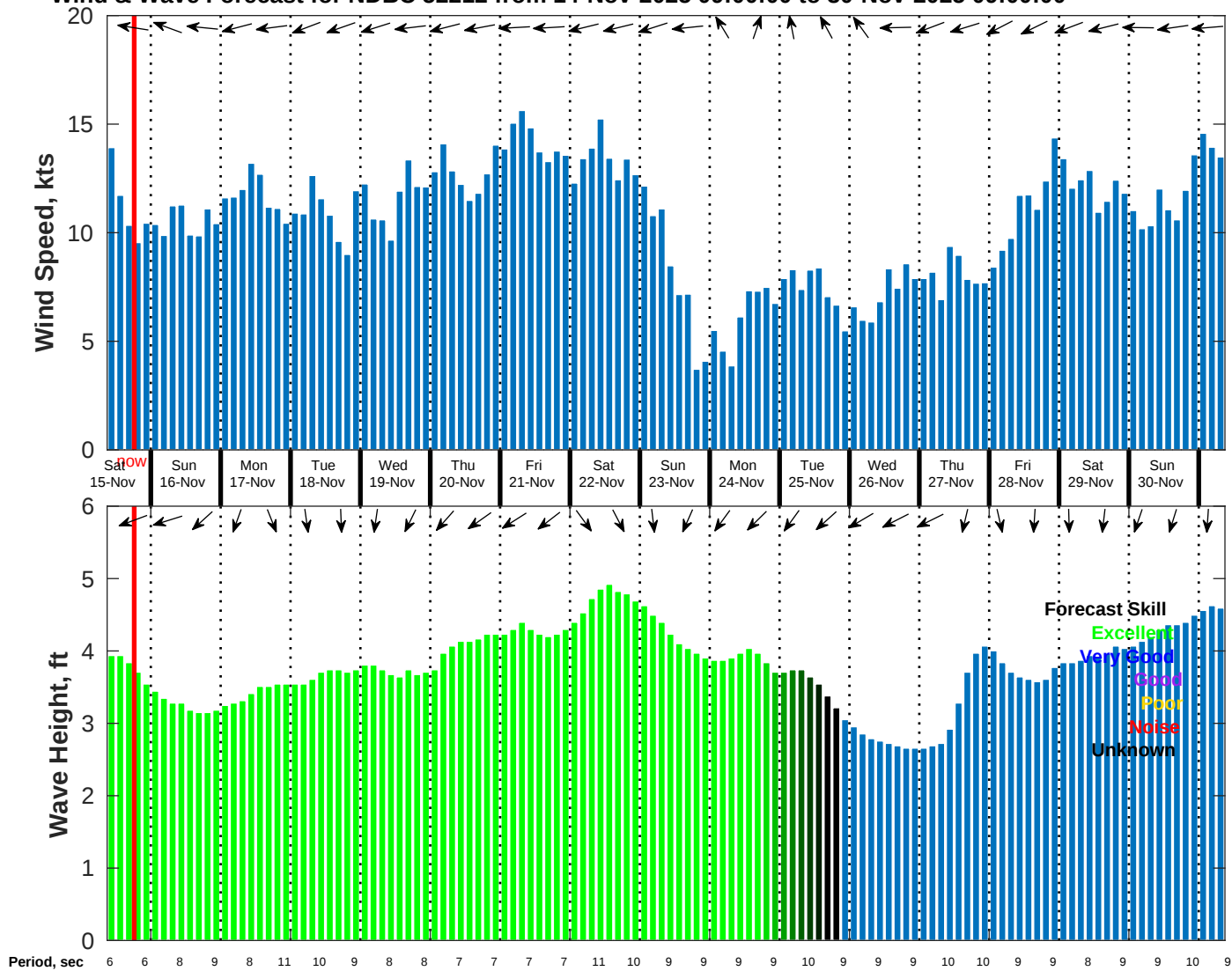
Wind & Wave Forecast for NDBC 52212 from 14-Nov-2025 09:00:00 to 30-Nov-2025 09:00:00
