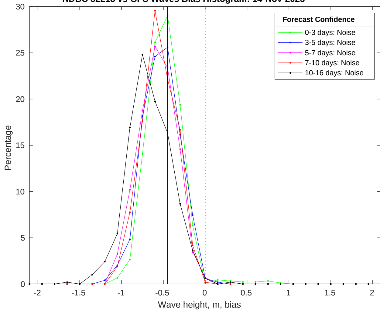
NDBC 52213 vs GFS Waves Bias Histogram: 14-Nov-2025
