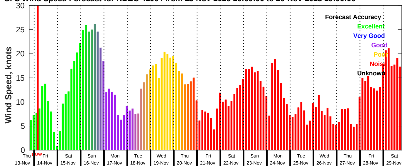
GFS Wind Speed Forecast for NDBC 41004 from 13-Nov-2025 19:00:00 to 29-Nov-2025 19:00:00
