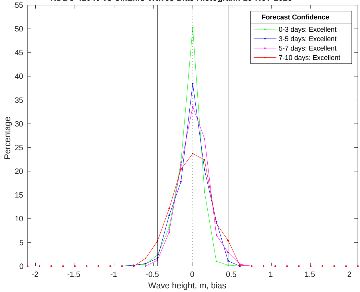
NDBC 41040 vs CMEMS Waves Bias Histogram: 15-Nov-2025
