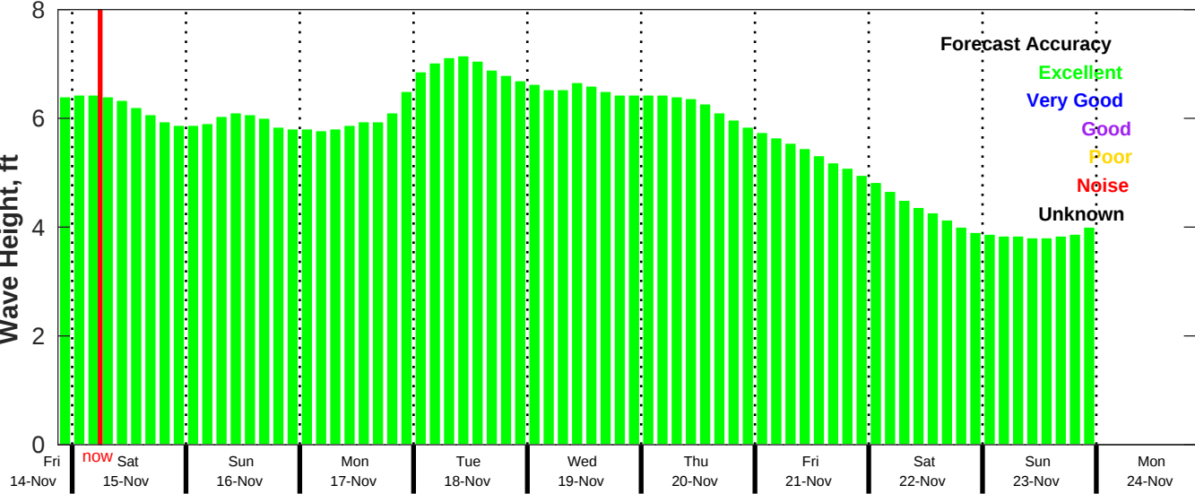
CMEMS Wave Forecast for NDBC 41040 from 14-Nov-2025 21:00:00 to 24-Nov-2025 21:00:00
