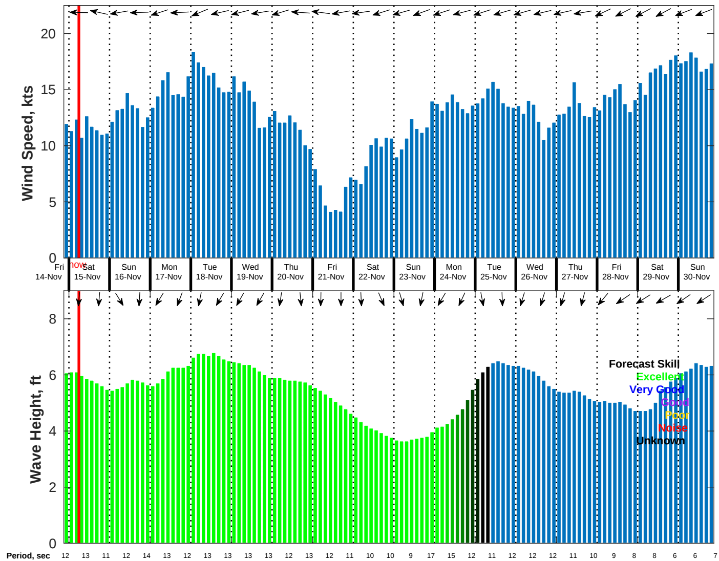
Wind & Wave Forecast for NDBC 41040 from 14-Nov-2025 21:00:00 to 30-Nov-2025 21:00:00
