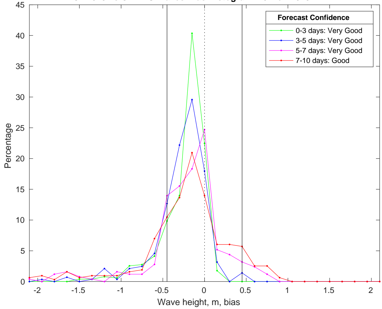
NDBC 42019 vs CMEMS Waves Bias Histogram: 15-Nov-2025
