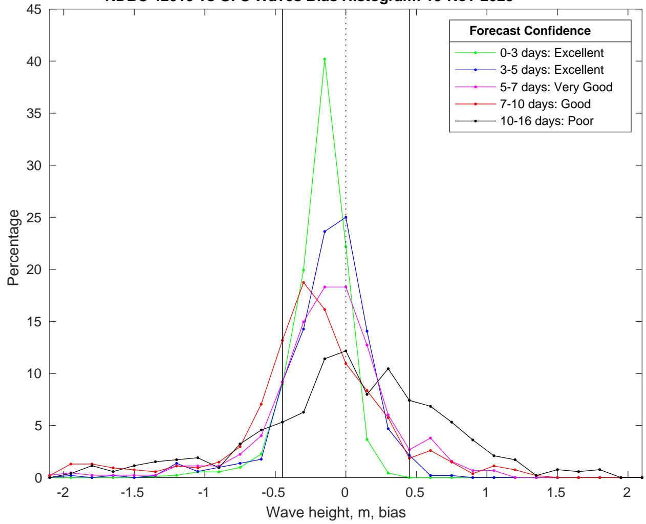
NDBC 42019 vs GFS Waves Bias Histogram: 15-Nov-2025
