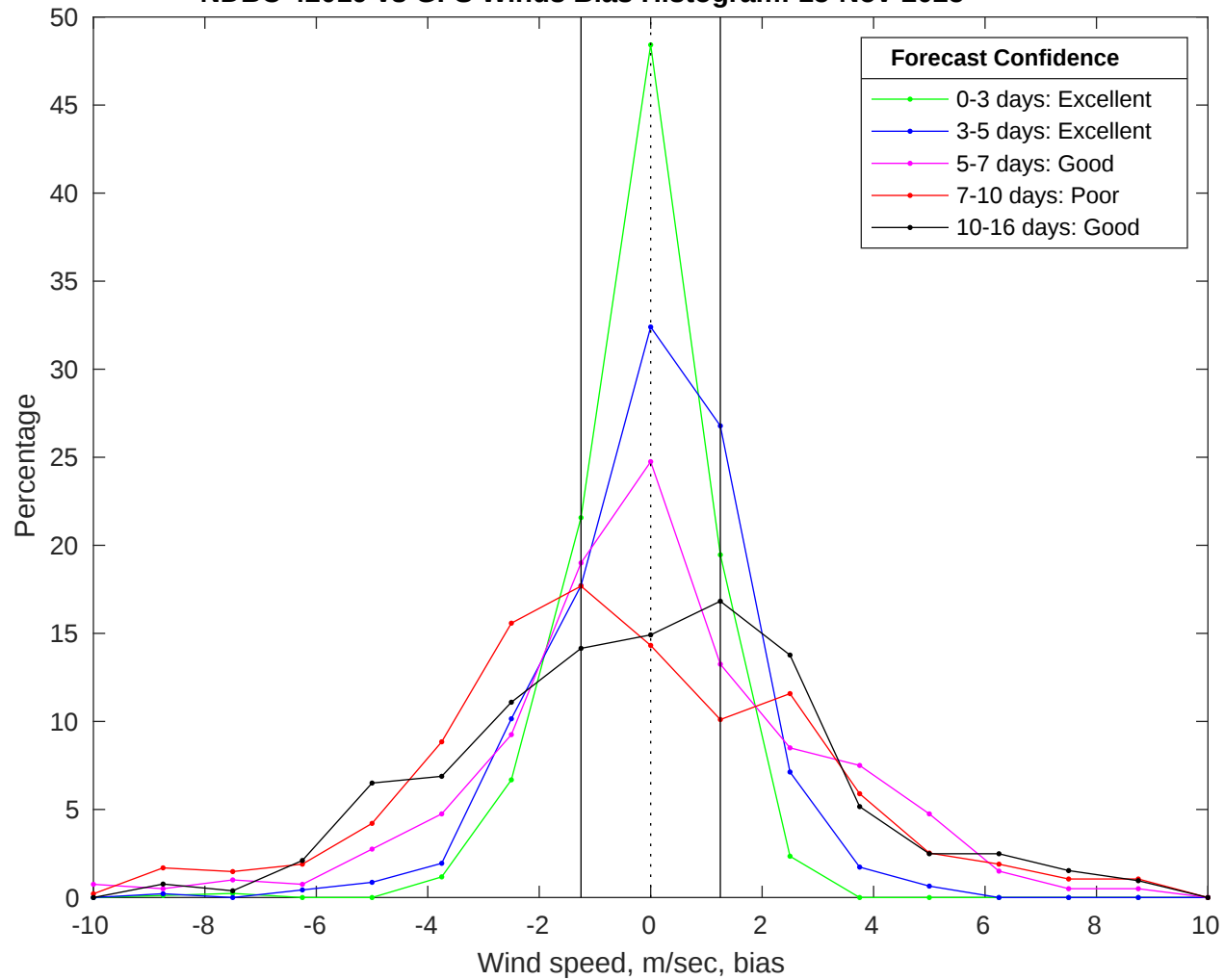
NDBC 42019 vs GFS Winds Bias Histogram: 15-Nov-2025
