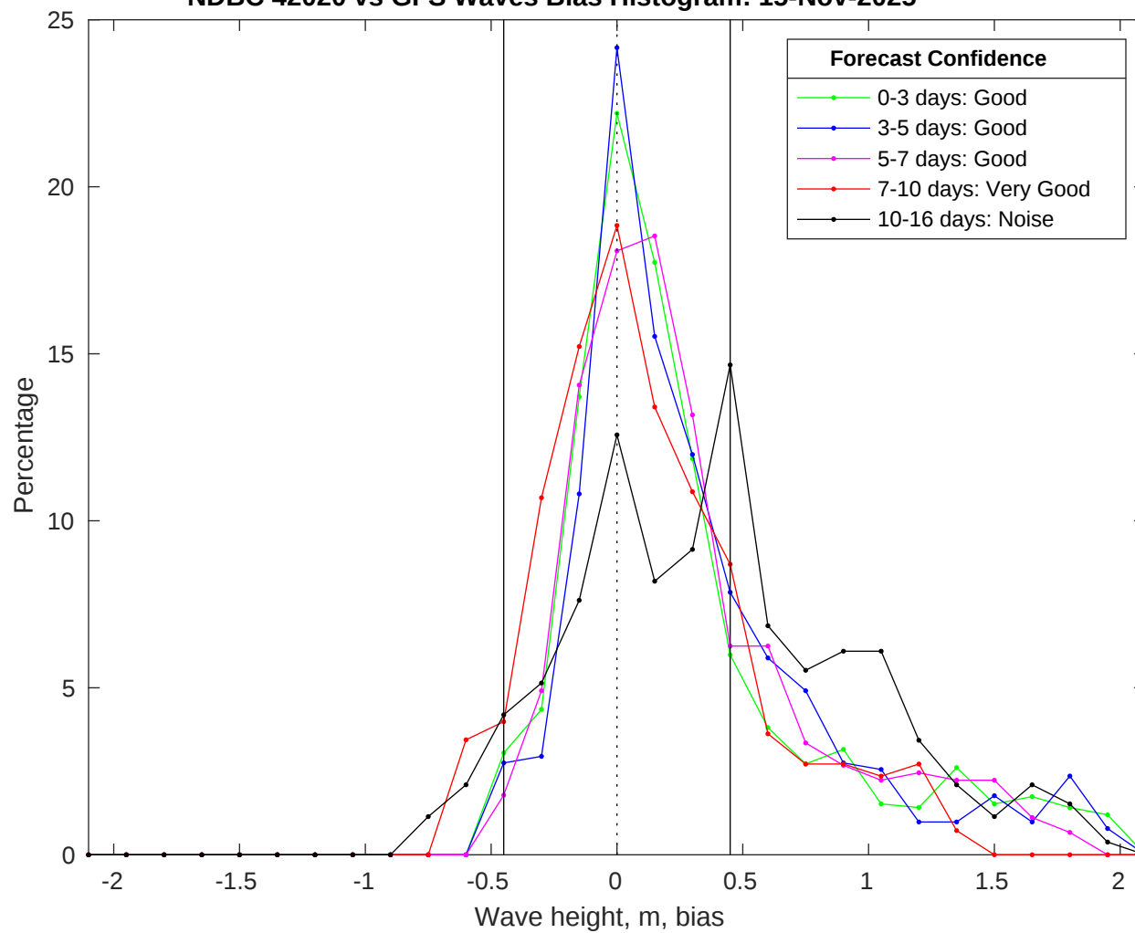
NDBC 42020 vs GFS Waves Bias Histogram: 15-Nov-2025
