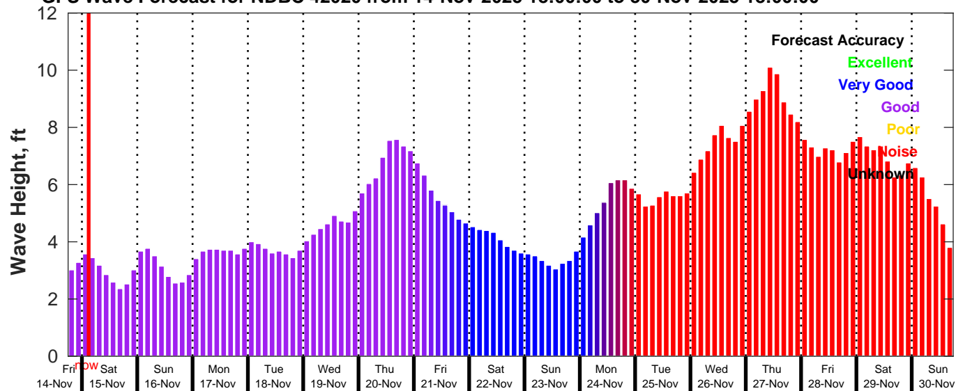
GFS Wave Forecast for NDBC 42020 from 14-Nov-2025 18:00:00 to 30-Nov-2025 18:00:00
