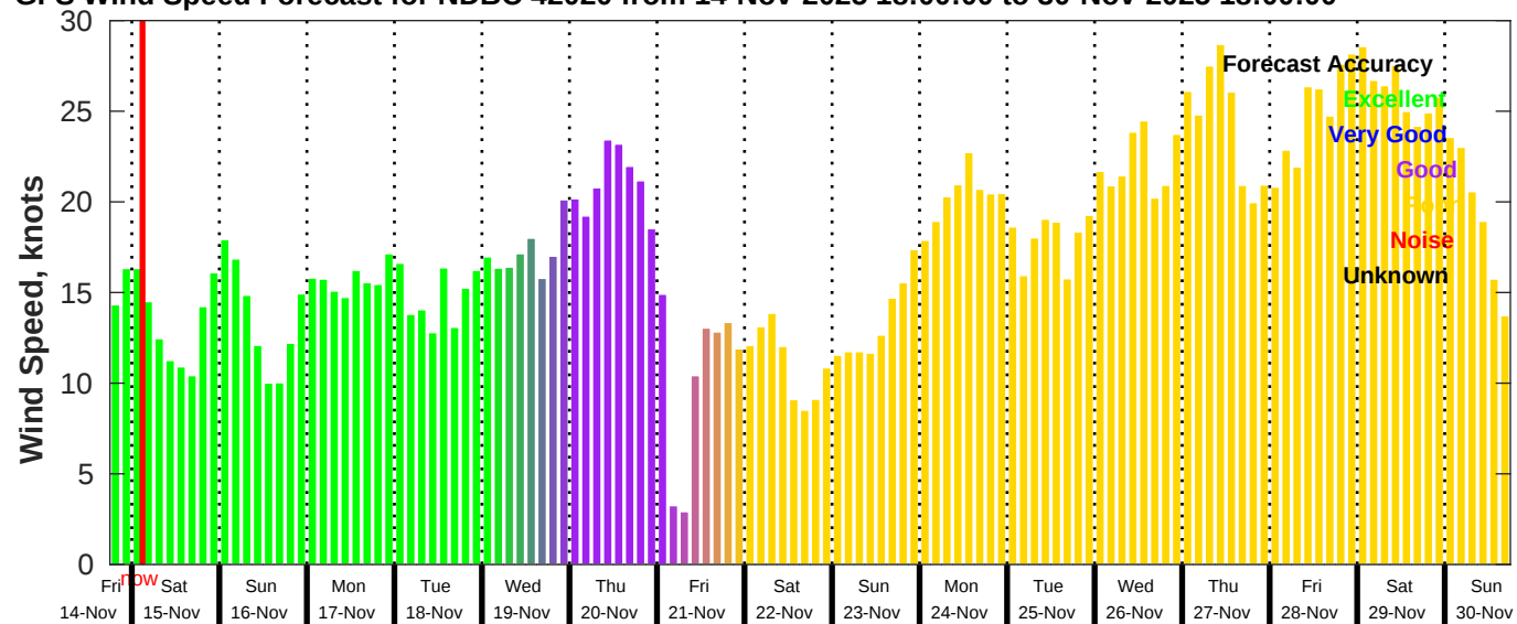
GFS Wind Speed Forecast for NDBC 42020 from 14-Nov-2025 18:00:00 to 30-Nov-2025 18:00:00
