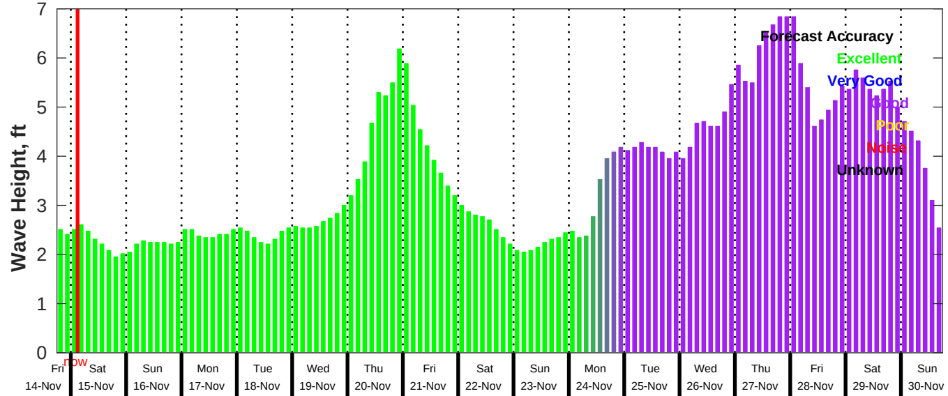
GFS Wave Forecast for NDBC 42035 from 14-Nov-2025 18:00:00 to 30-Nov-2025 18:00:00
