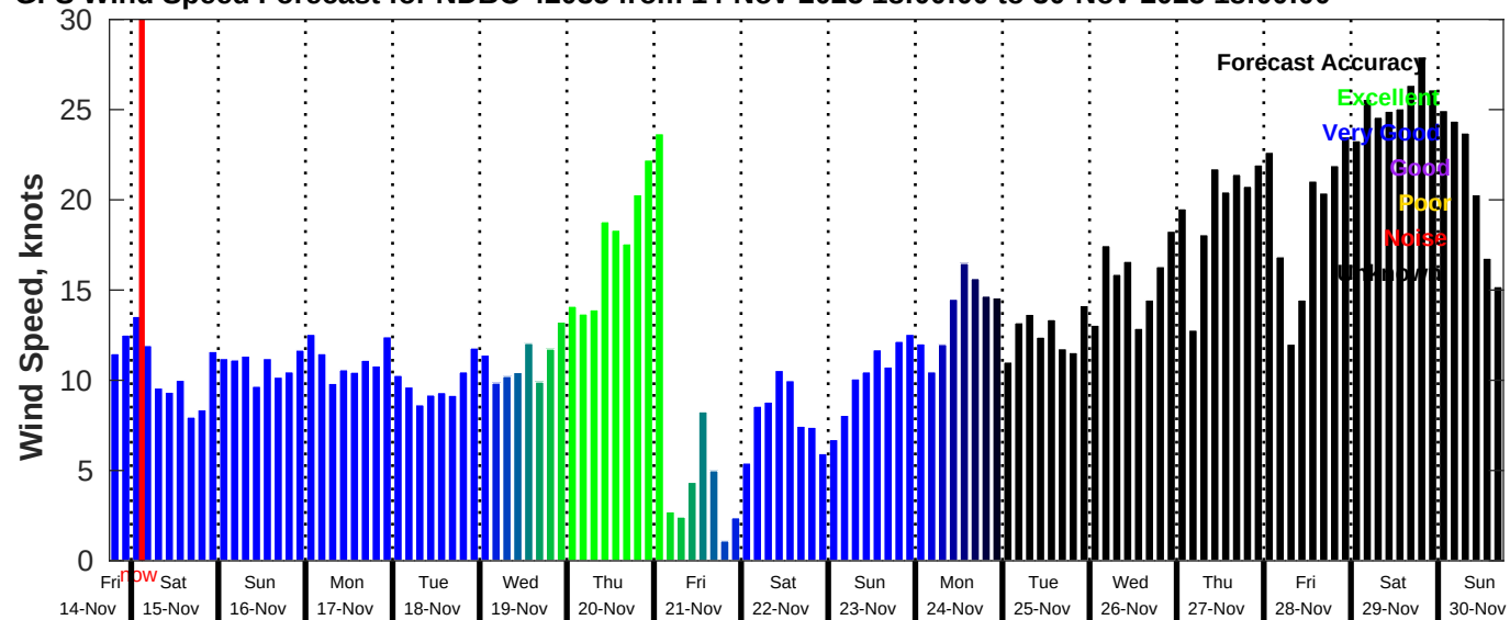
GFS Wind Speed Forecast for NDBC 42035 from 14-Nov-2025 18:00:00 to 30-Nov-2025 18:00:00
