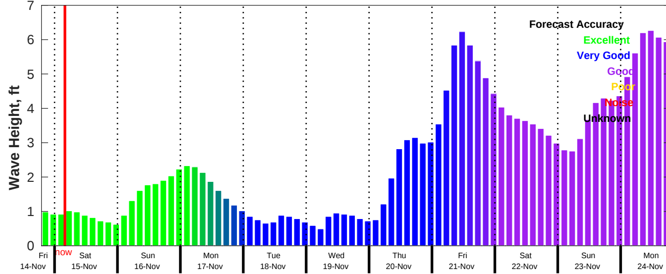
CMEMS Wave Forecast for NDBC 42036 from 14-Nov-2025 19:00:00 to 24-Nov-2025 19:00:00
