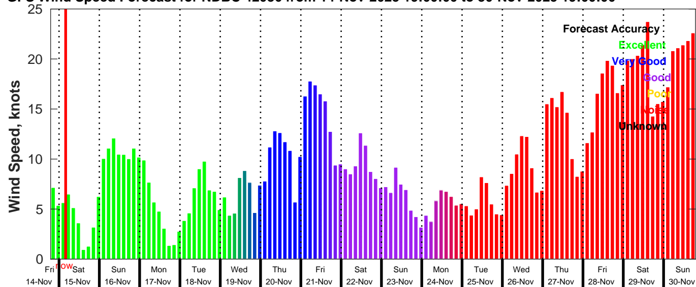
GFS Wind Speed Forecast for NDBC 42036 from 14-Nov-2025 19:00:00 to 30-Nov-2025 19:00:00
