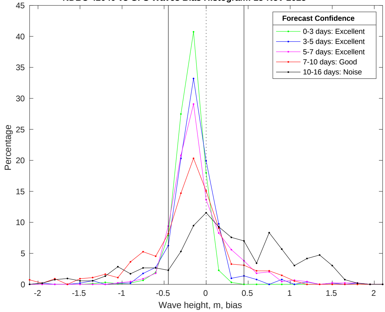
NDBC 42040 vs GFS Waves Bias Histogram: 15-Nov-2025
