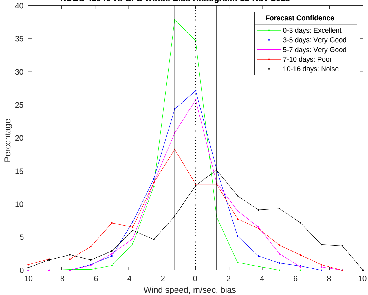
NDBC 42040 vs GFS Winds Bias Histogram: 15-Nov-2025
