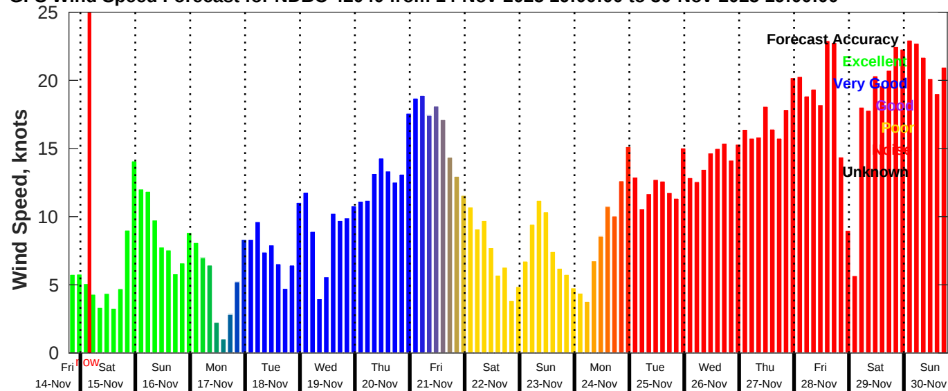
GFS Wind Speed Forecast for NDBC 42040 from 14-Nov-2025 19:00:00 to 30-Nov-2025 19:00:00
