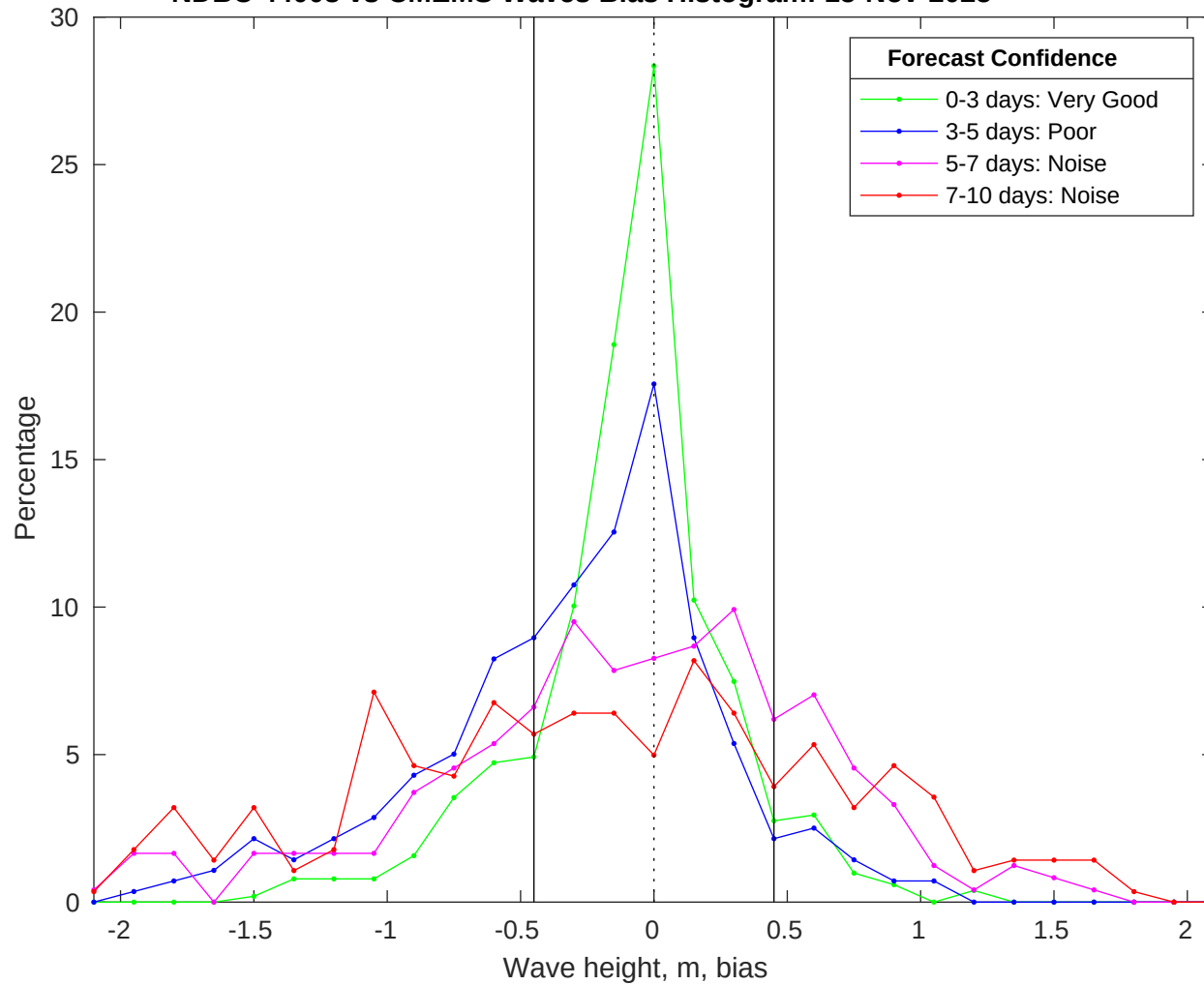
NDBC 44008 vs CMEMS Waves Bias Histogram: 15-Nov-2025
