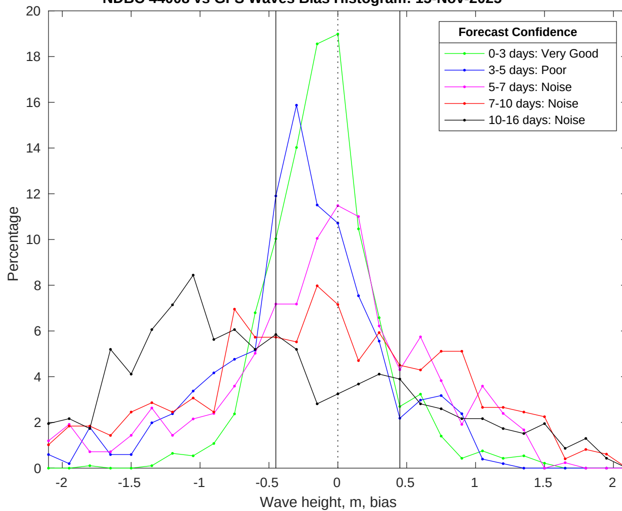
NDBC 44008 vs GFS Waves Bias Histogram: 15-Nov-2025
