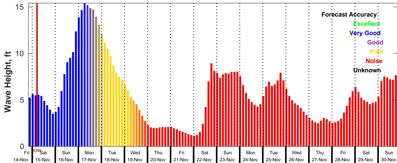
GFS Wave Forecast for NDBC 44008 from 14-Nov-2025 20:00:00 to 30-Nov-2025 20:00:00
