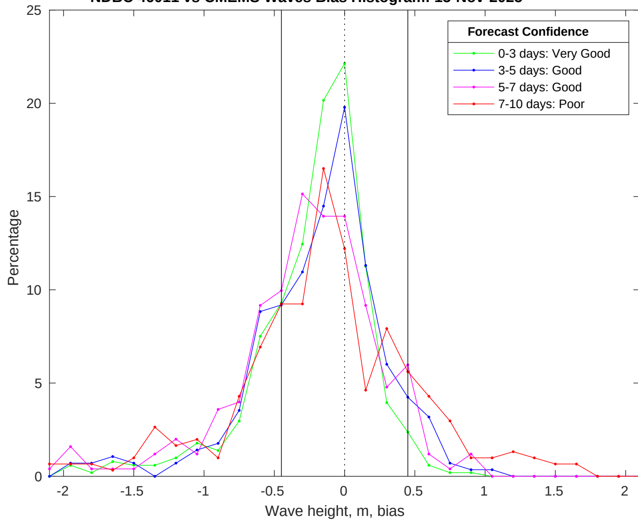
NDBC 46011 vs CMEMS Waves Bias Histogram: 15-Nov-2025
