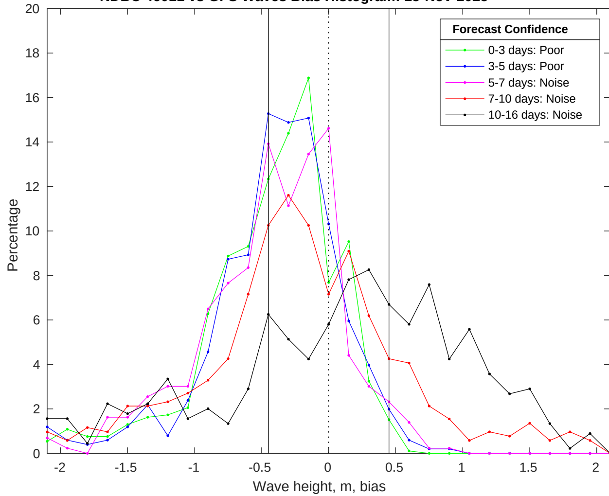
NDBC 46011 vs GFS Waves Bias Histogram: 15-Nov-2025
