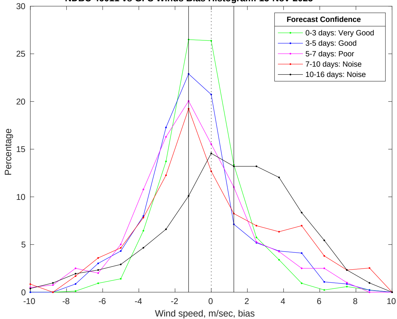
NDBC 46011 vs GFS Winds Bias Histogram: 15-Nov-2025
