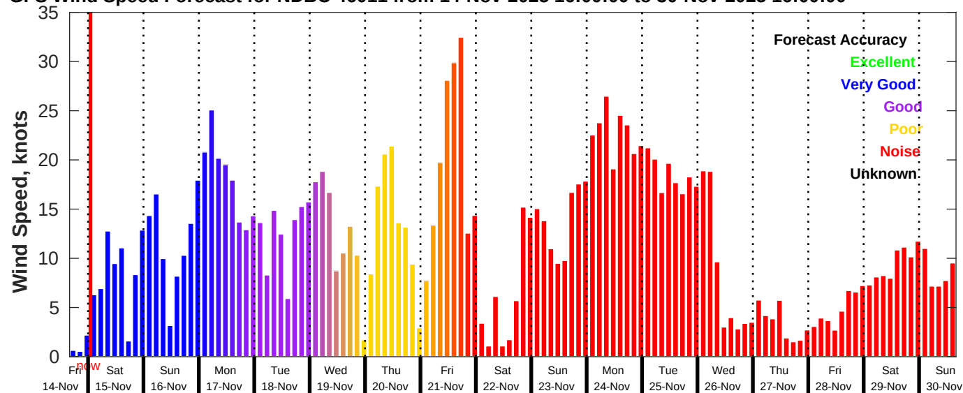
GFS Wind Speed Forecast for NDBC 46011 from 14-Nov-2025 16:00:00 to 30-Nov-2025 16:00:00
