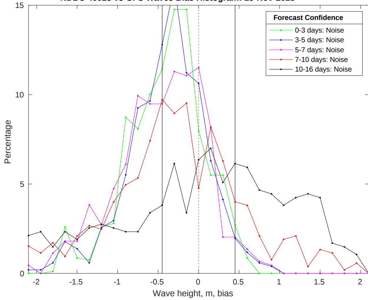
NDBC 46028 vs GFS Waves Bias Histogram: 15-Nov-2025
