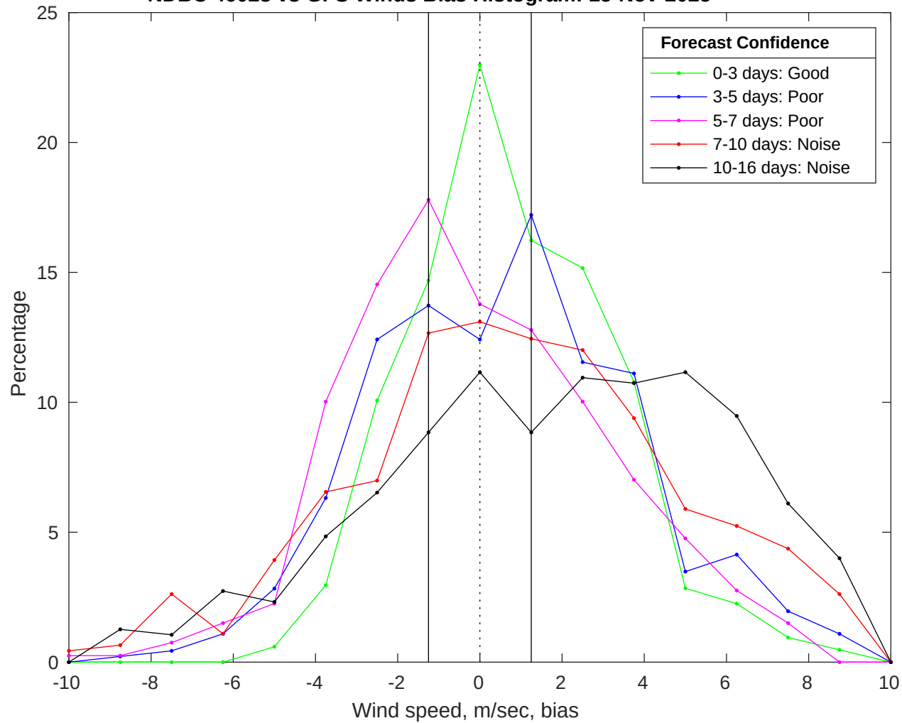
NDBC 46028 vs GFS Winds Bias Histogram: 15-Nov-2025
