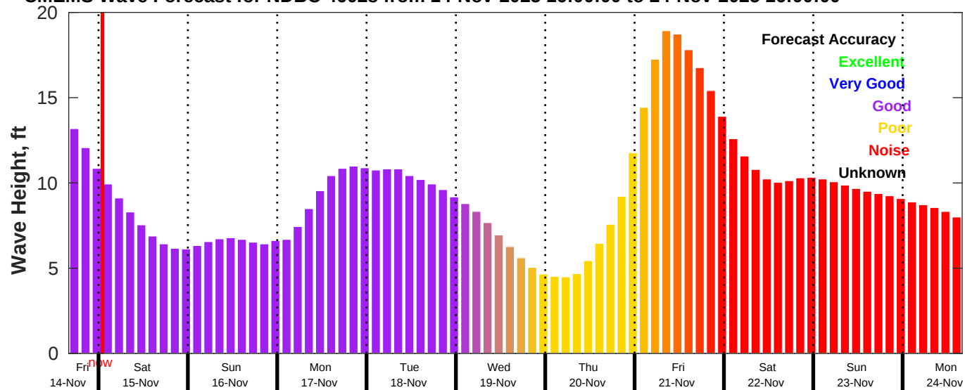
CMEMS Wave Forecast for NDBC 46028 from 14-Nov-2025 16:00:00 to 24-Nov-2025 16:00:00
