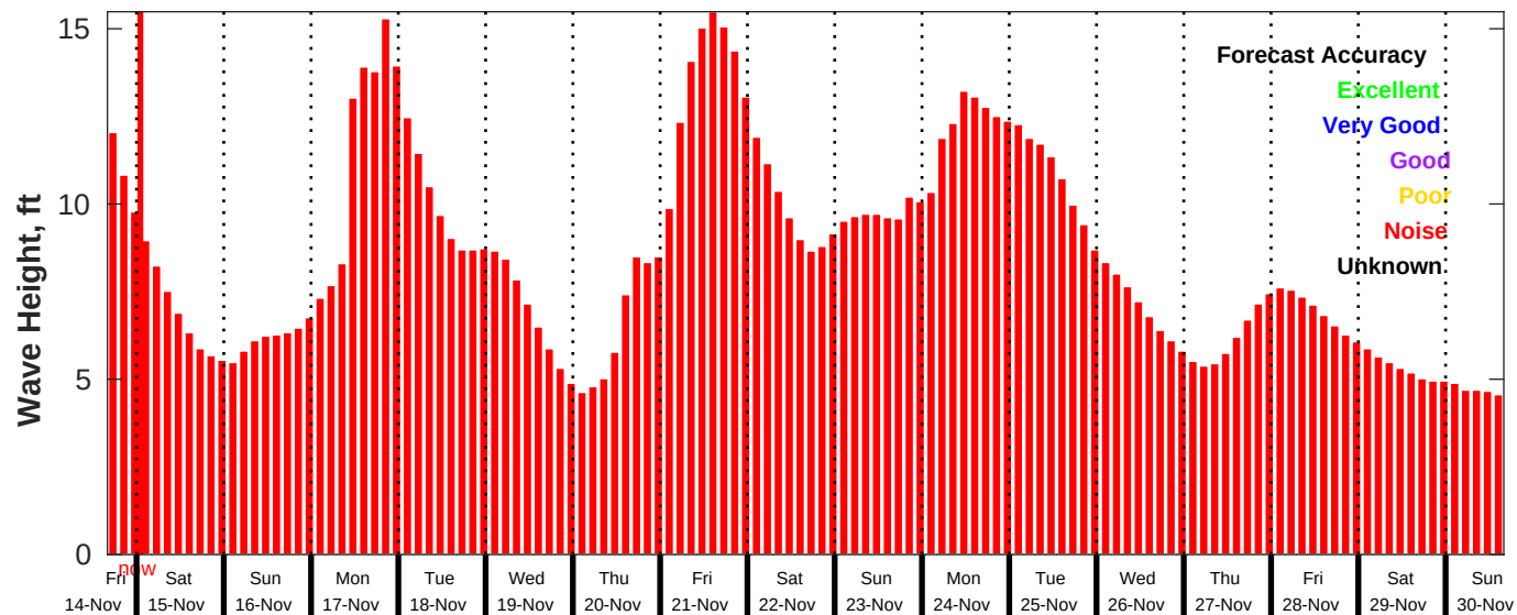
GFS Wave Forecast for NDBC 46028 from 14-Nov-2025 16:00:00 to 30-Nov-2025 16:00:00
