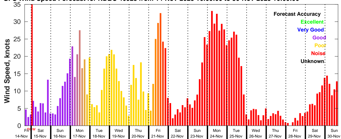
GFS Wind Speed Forecast for NDBC 46028 from 14-Nov-2025 16:00:00 to 30-Nov-2025 16:00:00
