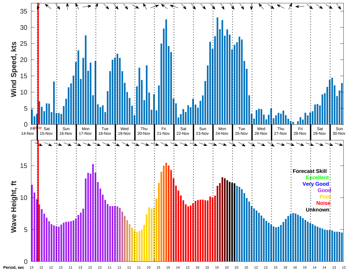
Wind & Wave Forecast for NDBC 46028 from 14-Nov-2025 16:00:00 to 30-Nov-2025 16:00:00
