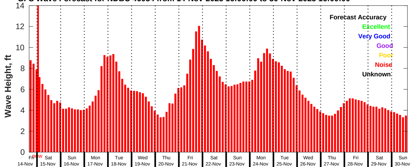
GFS Wave Forecast for NDBC 46054 from 14-Nov-2025 16:00:00 to 30-Nov-2025 16:00:00
