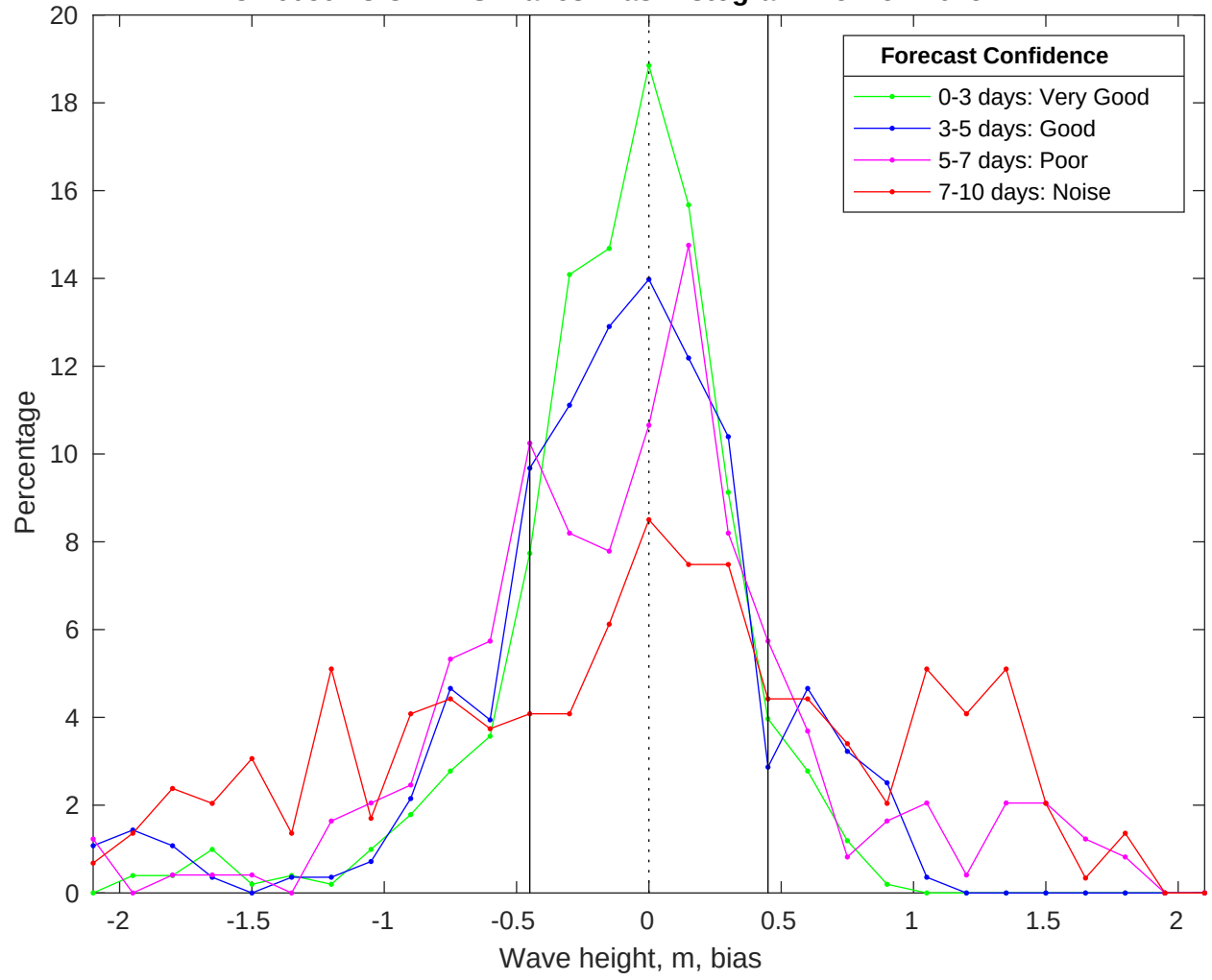
NDBC 46059 vs CMEMS Waves Bias Histogram: 15-Nov-2025
