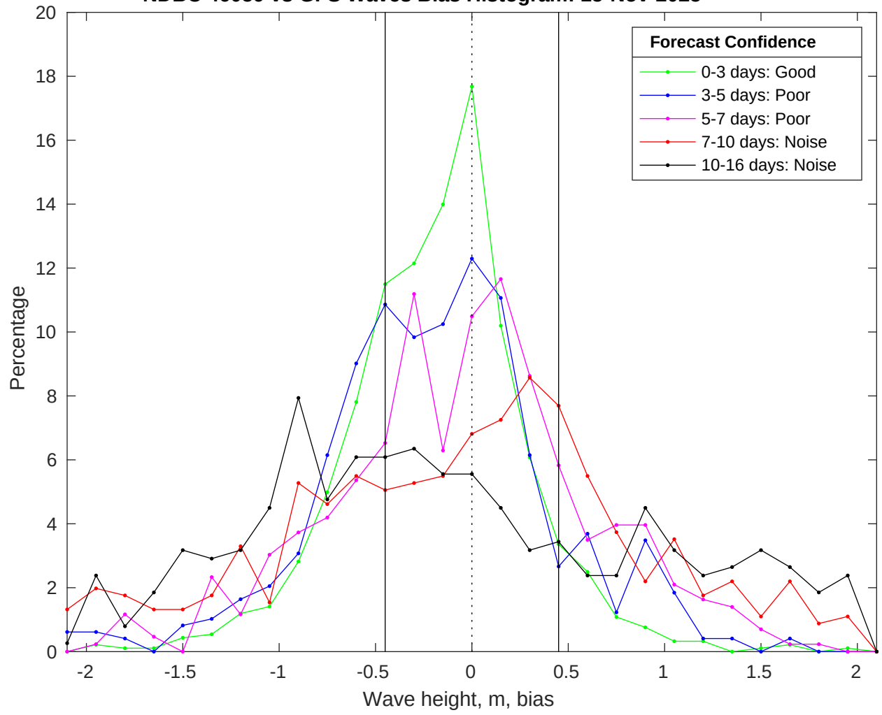
NDBC 46059 vs GFS Waves Bias Histogram: 15-Nov-2025
