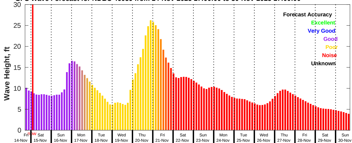
GFS Wave Forecast for NDBC 46059 from 14-Nov-2025 17:00:00 to 30-Nov-2025 17:00:00
