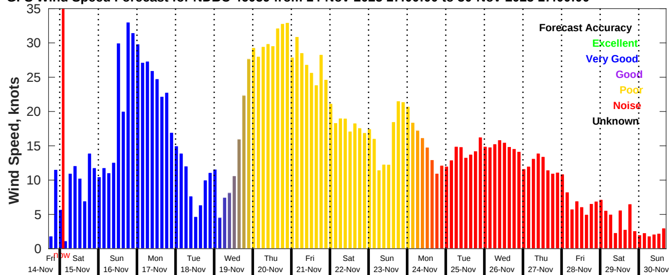
GFS Wind Speed Forecast for NDBC 46059 from 14-Nov-2025 17:00:00 to 30-Nov-2025 17:00:00
