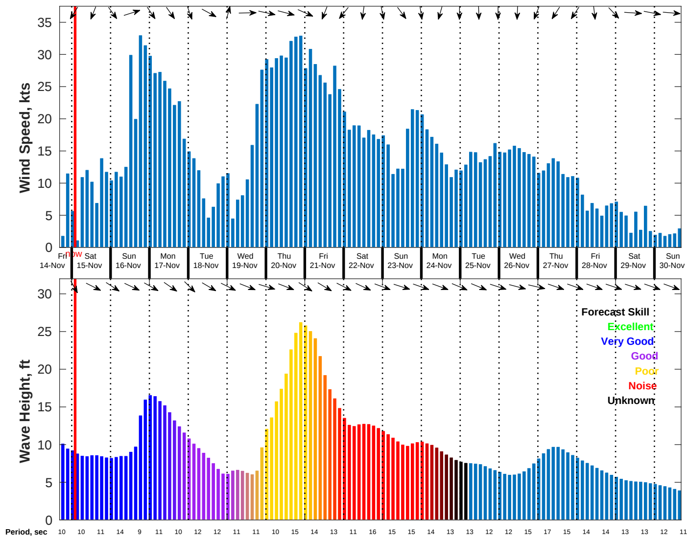
Wind & Wave Forecast for NDBC 46059 from 14-Nov-2025 17:00:00 to 30-Nov-2025 17:00:00
