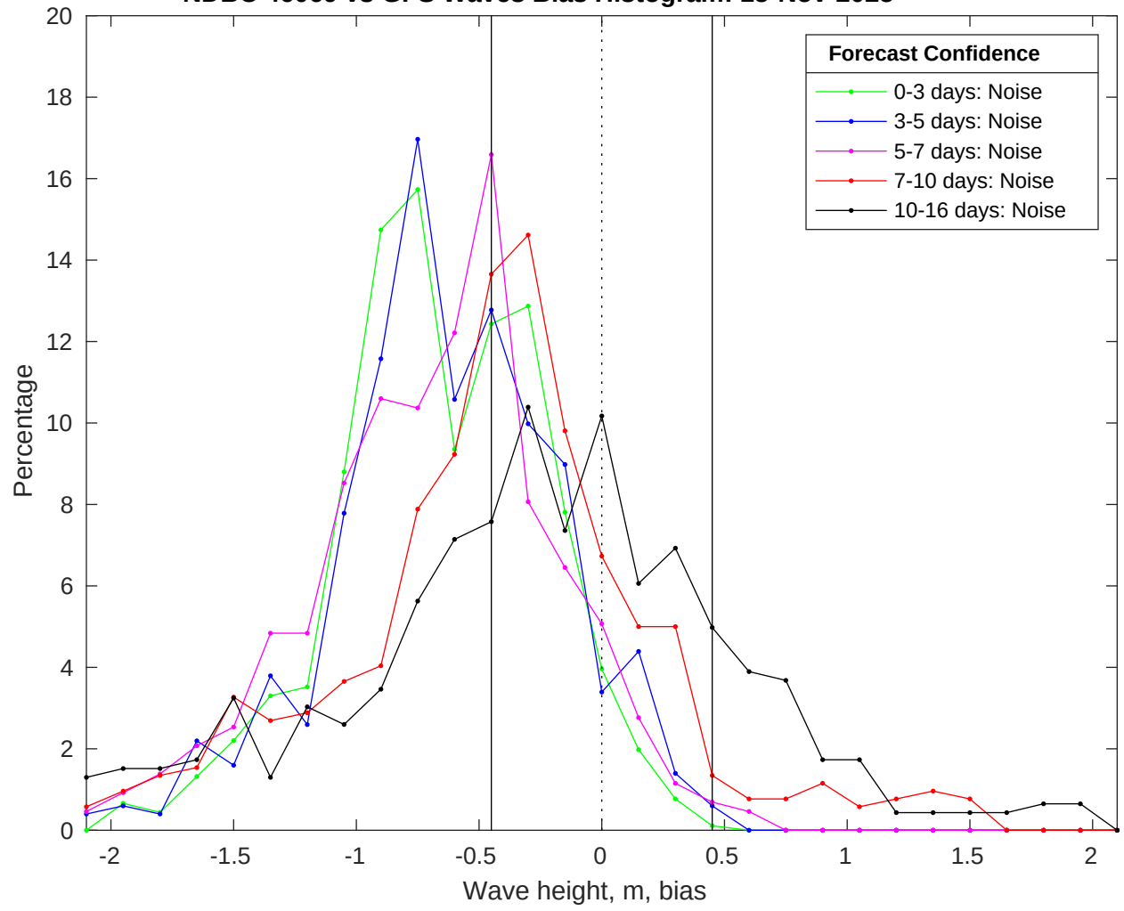
NDBC 46069 vs GFS Waves Bias Histogram: 15-Nov-2025
