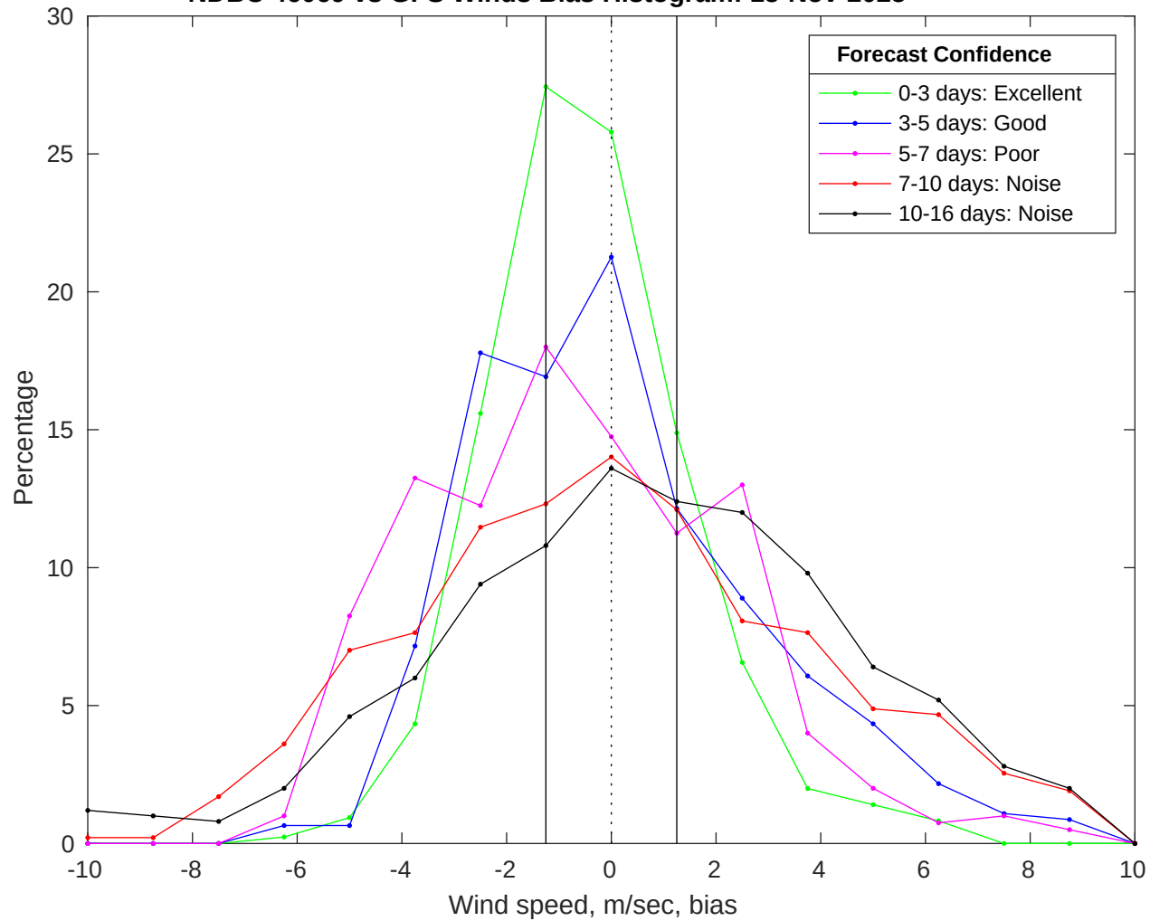
NDBC 46069 vs GFS Winds Bias Histogram: 15-Nov-2025
