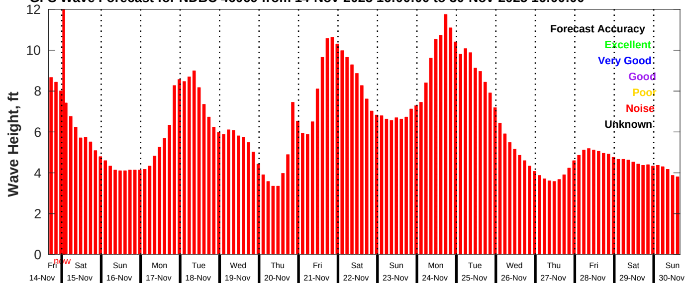
GFS Wave Forecast for NDBC 46069 from 14-Nov-2025 16:00:00 to 30-Nov-2025 16:00:00
