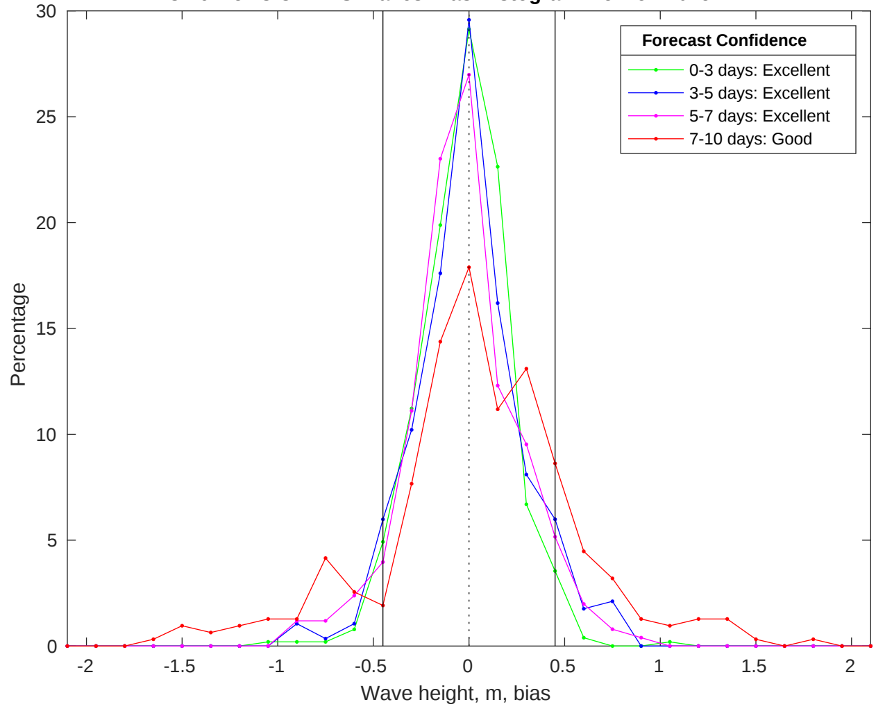
NDBC 46215 vs CMEMS Waves Bias Histogram: 15-Nov-2025
