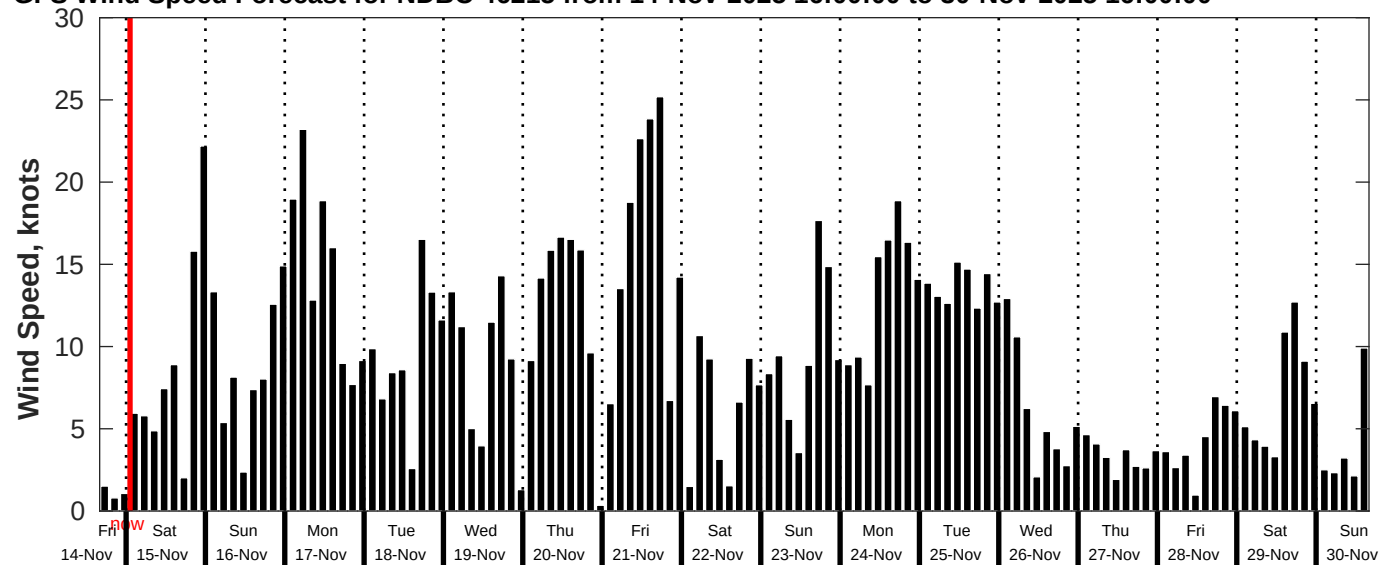
GFS Wind Speed Forecast for NDBC 46215 from 14-Nov-2025 16:00:00 to 30-Nov-2025 16:00:00
