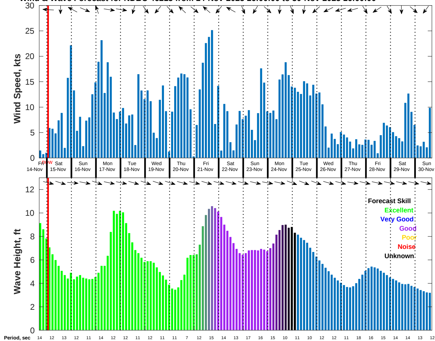
Wind & Wave Forecast for NDBC 46215 from 14-Nov-2025 16:00:00 to 30-Nov-2025 16:00:00
