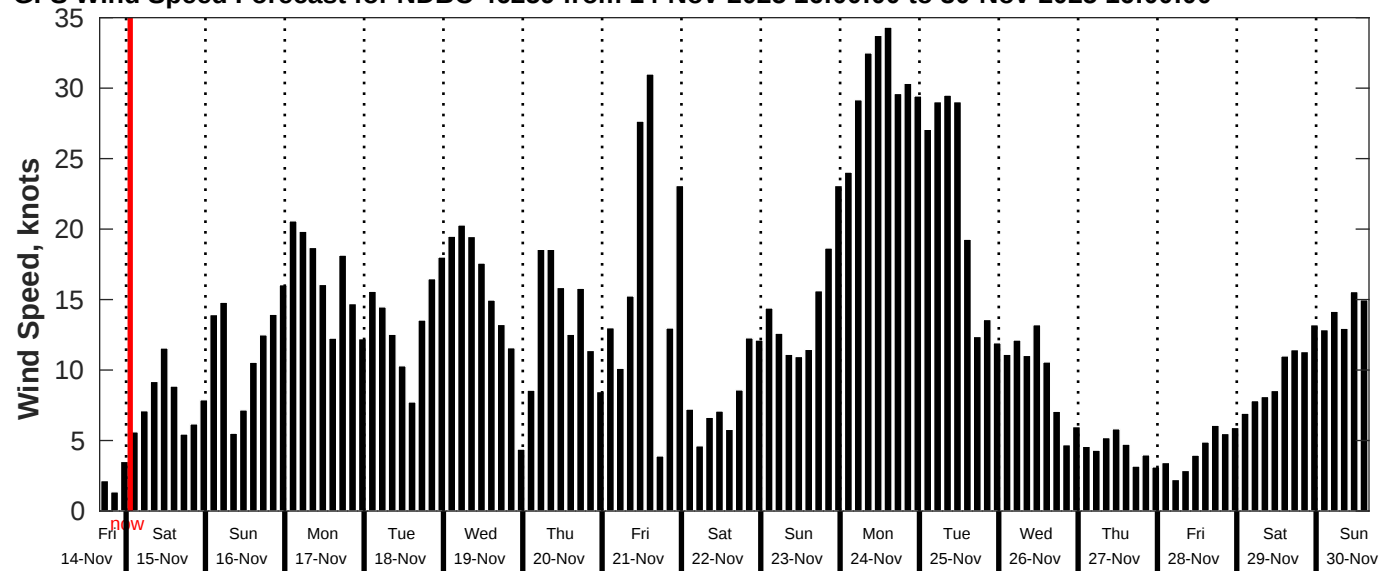
GFS Wind Speed Forecast for NDBC 46259 from 14-Nov-2025 16:00:00 to 30-Nov-2025 16:00:00
