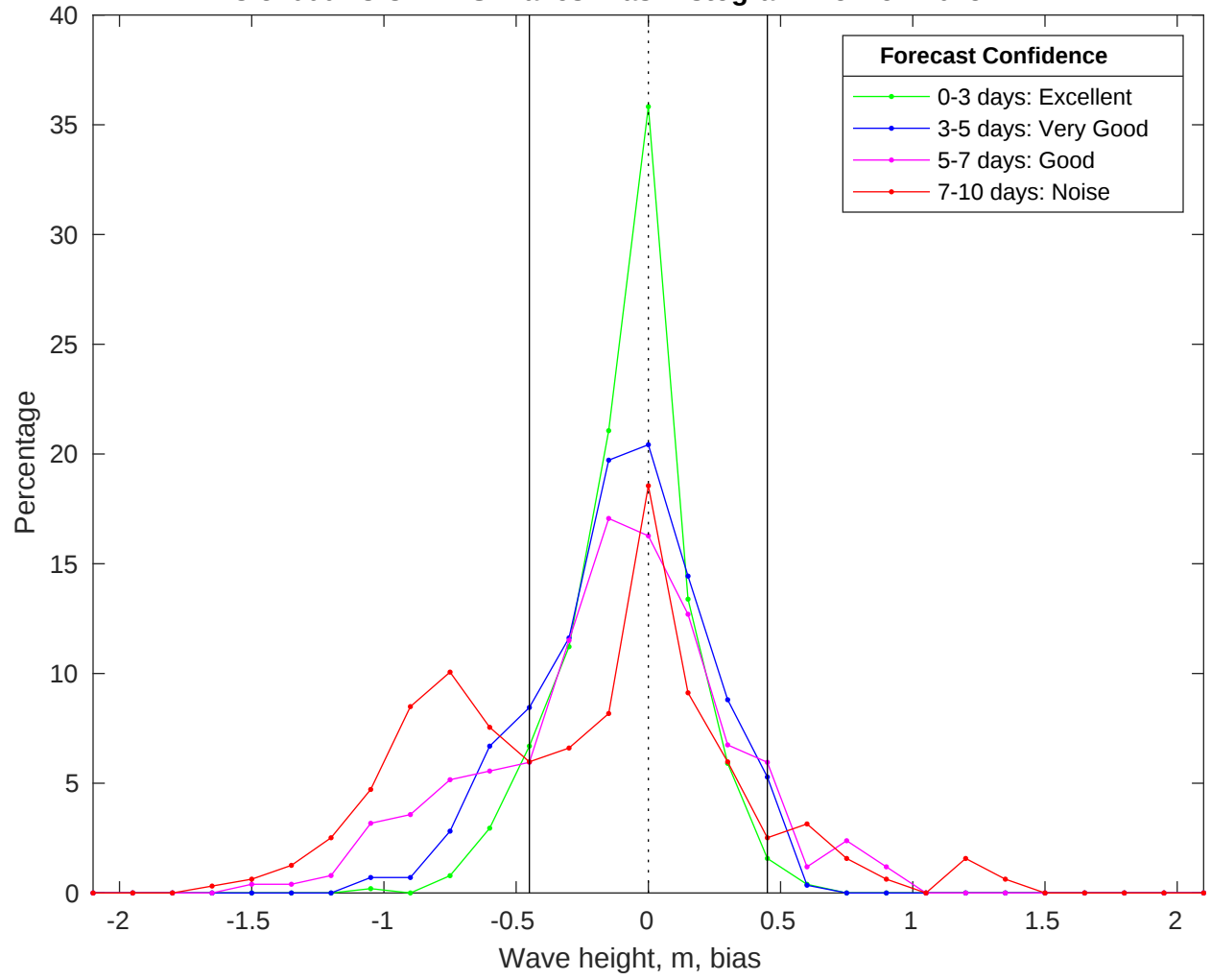
NDBC 51000 vs CMEMS Waves Bias Histogram: 15-Nov-2025
