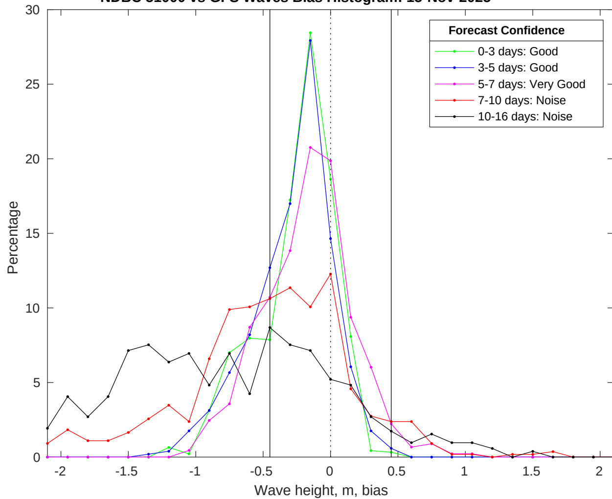
NDBC 51000 vs GFS Waves Bias Histogram: 15-Nov-2025
