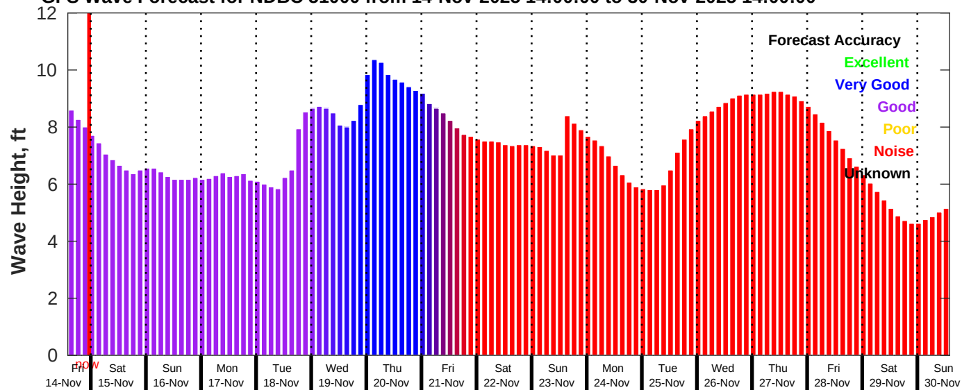
GFS Wave Forecast for NDBC 51000 from 14-Nov-2025 14:00:00 to 30-Nov-2025 14:00:00
