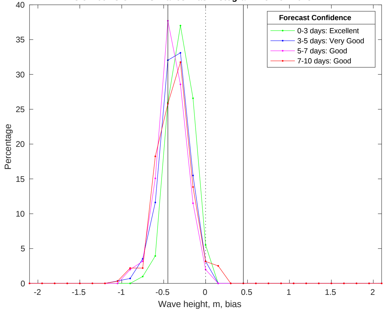
NDBC 51209 vs CMEMS Waves Bias Histogram: 15-Nov-2025
