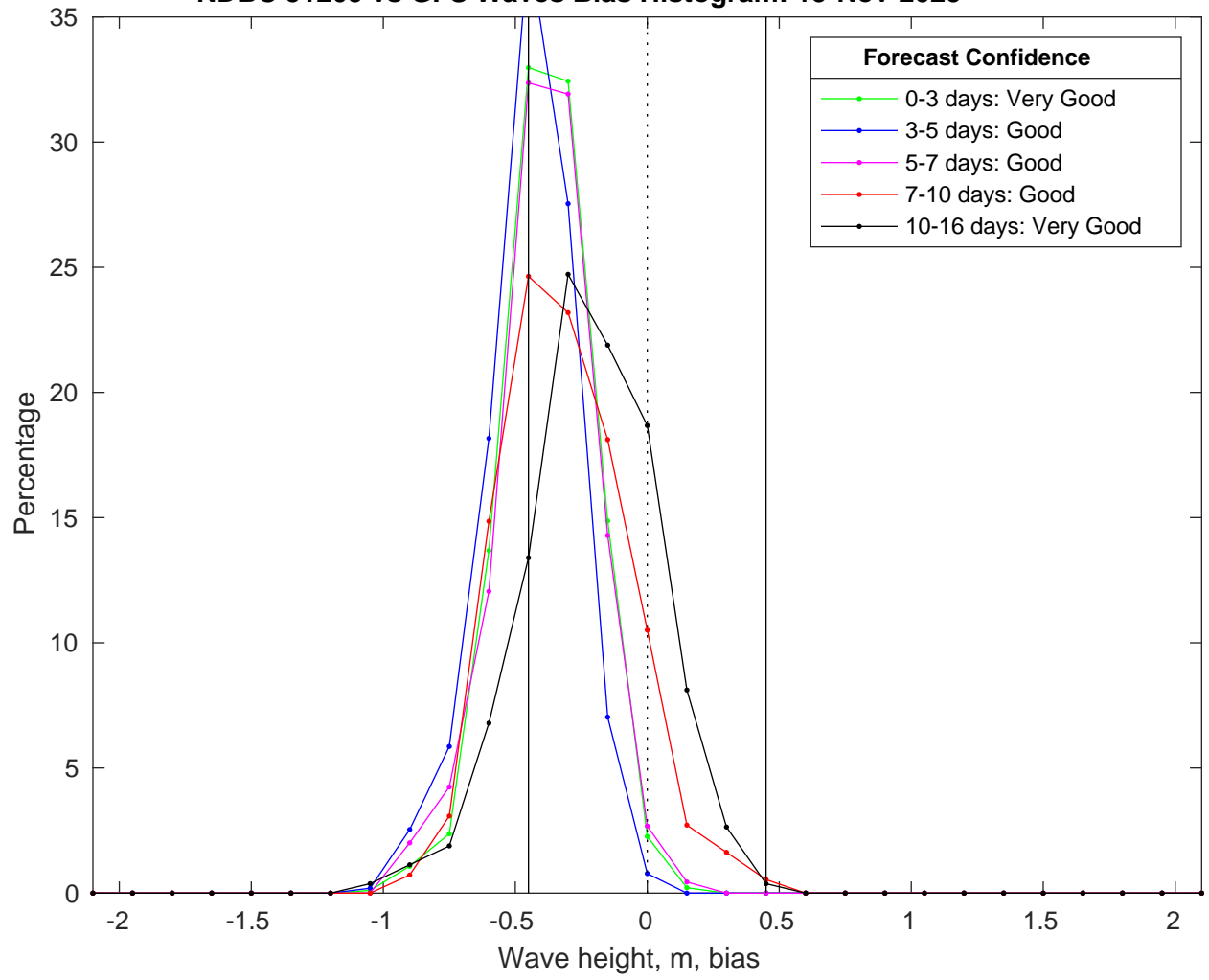
NDBC 51209 vs GFS Waves Bias Histogram: 15-Nov-2025
